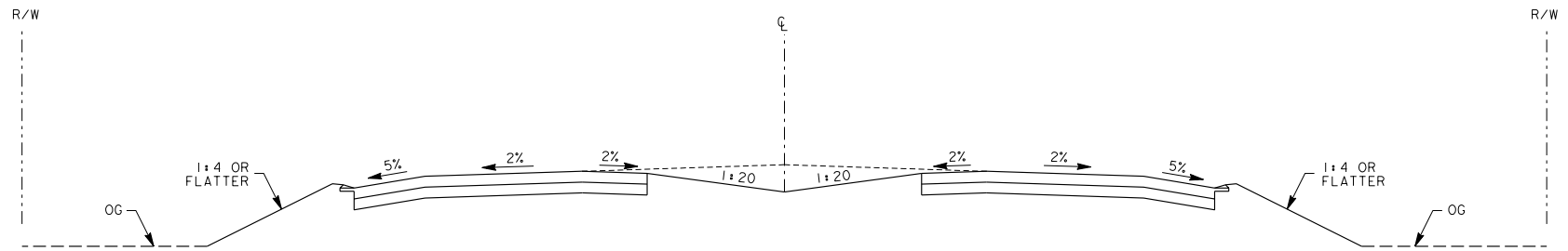
TYPICAL CROSS SECTION SR 79 NTS LIMITED ACCESS EXPRESSWAY
